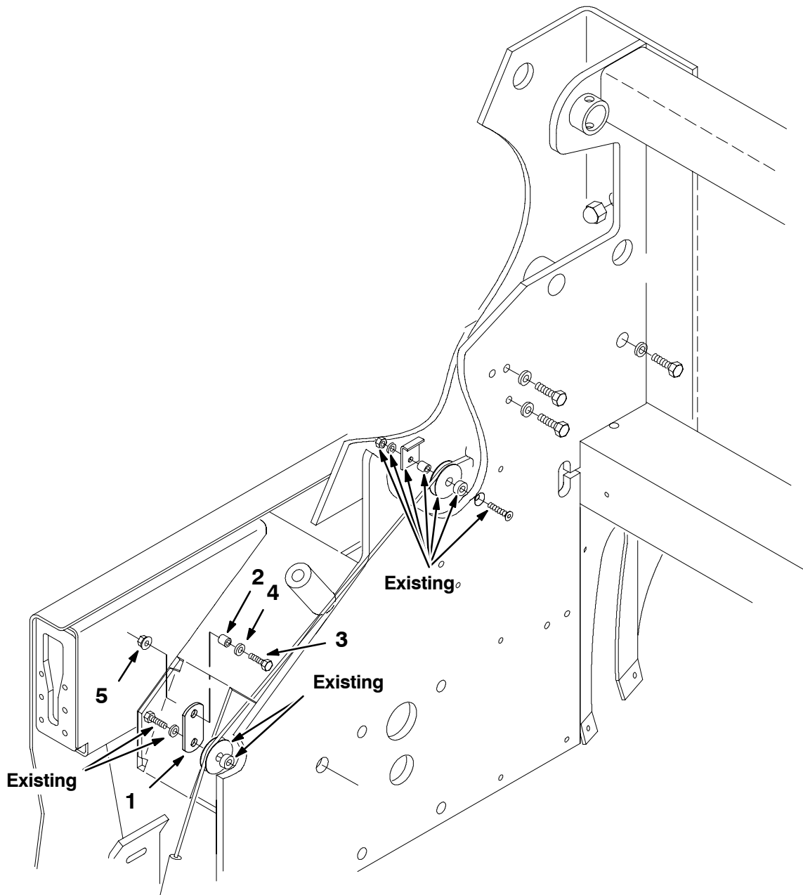
FIG. 2 – New Side Brush Lift Cable and Pulley Assembly
