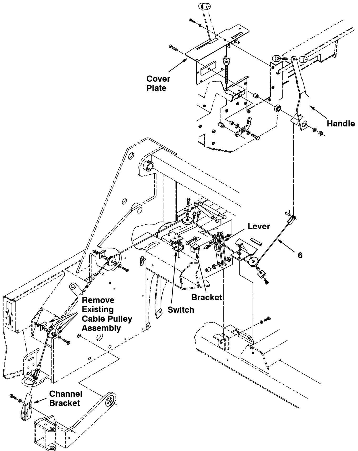
FIG. 1 – Existing Cable Keeper Bracket Assembly
